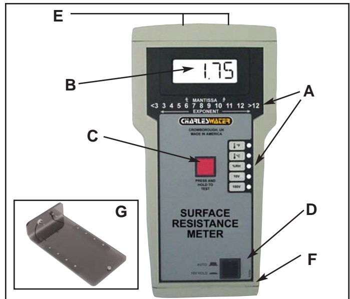
Figure 2. Features of the Surface Resistance Meter
