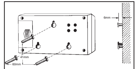
Figure 2. Mounting hole locations
