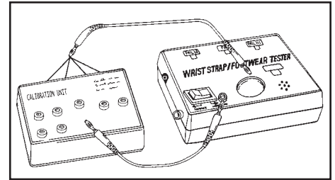
Figure 14. Calibration of the Combo Tester 750K to 35M range with the model 99090
