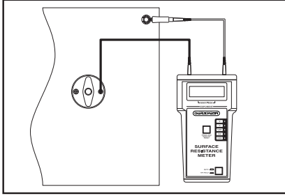
Figure 8. Proper connection of leads.
