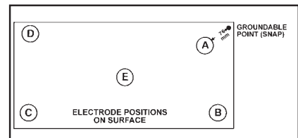
Figure 7. Electrode positions on surface of pad, Rg test.
