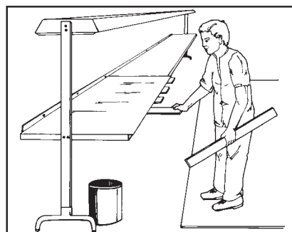
Figure 3. Micastat® sheet on wooden strips
