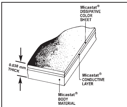
Figure 2. Micastat® layered construction
