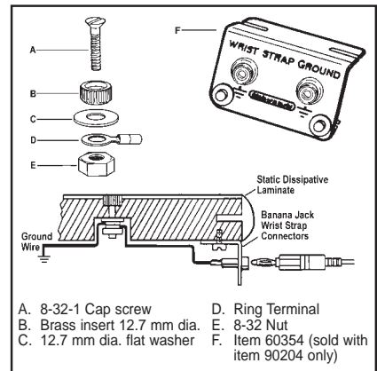
Figure 5. Component Parts and Installation of 90202 and 90204.
