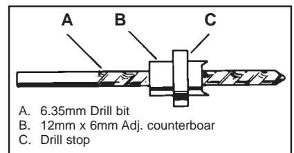
Figure 6. Drill Tool 90200.
